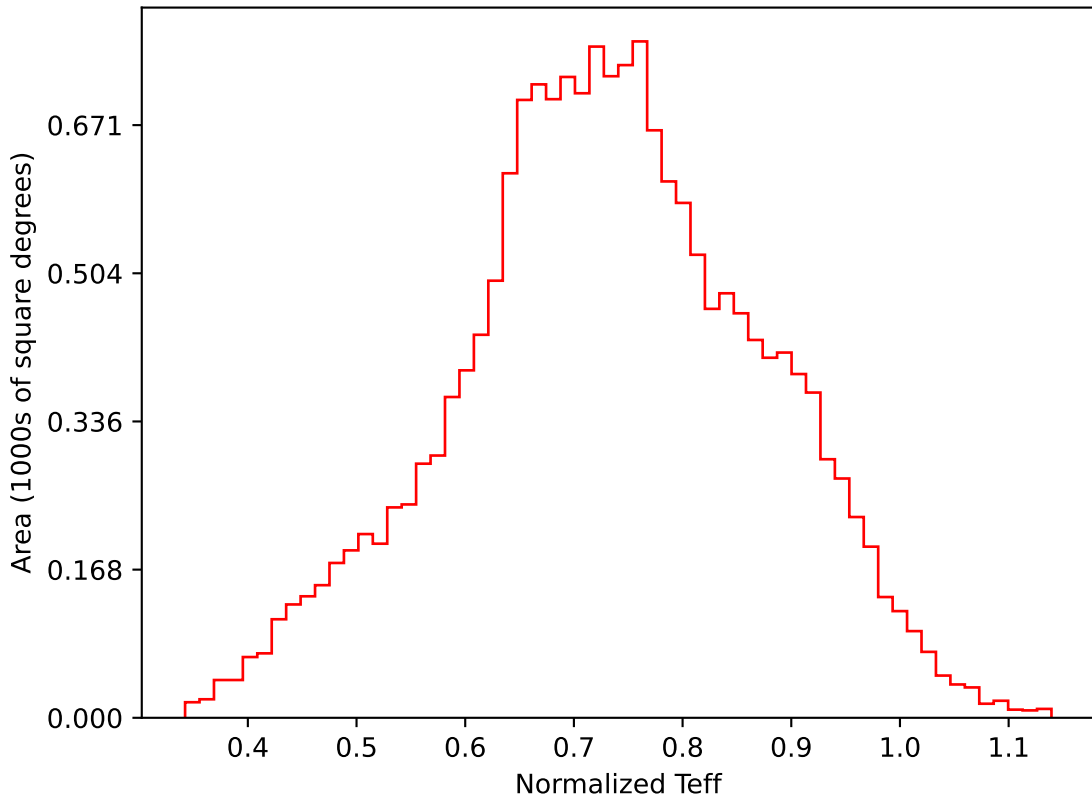
ddf_loaded_fl8_v3.4_10yrs WFD i band: Normalized Teff
