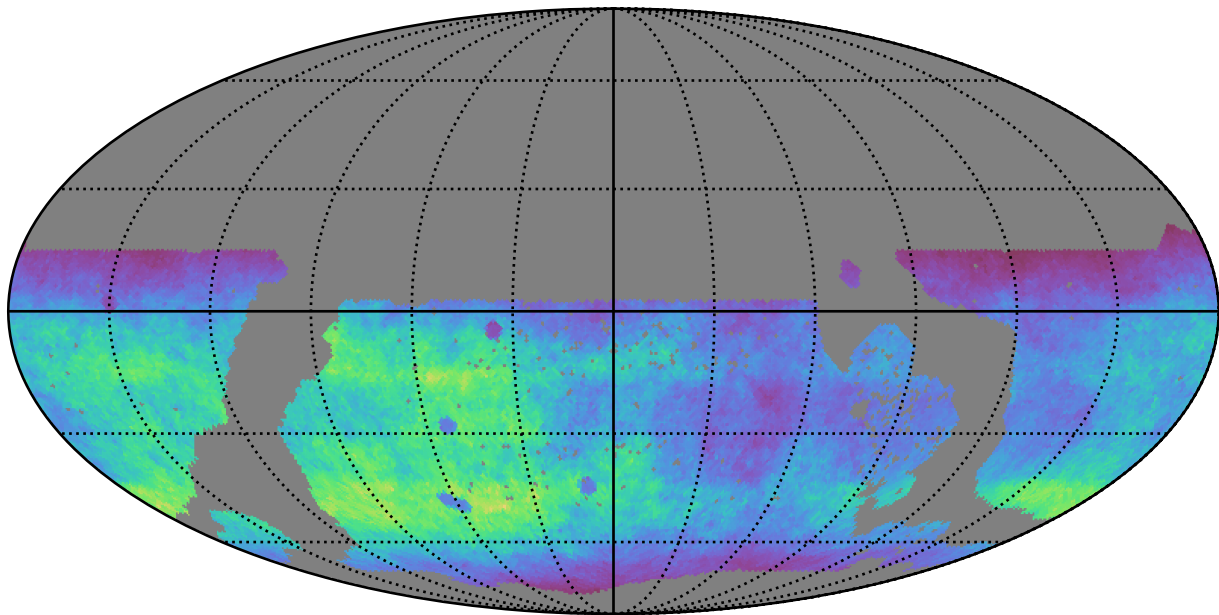
ddf_loaded_fl8_v3.4_10yrs WFD g band: Normalized Teff
