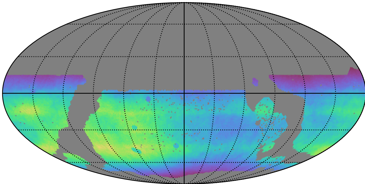
ddf_loaded_fl8_v3.4_10yrs WFD all bands: Normalized Teff
