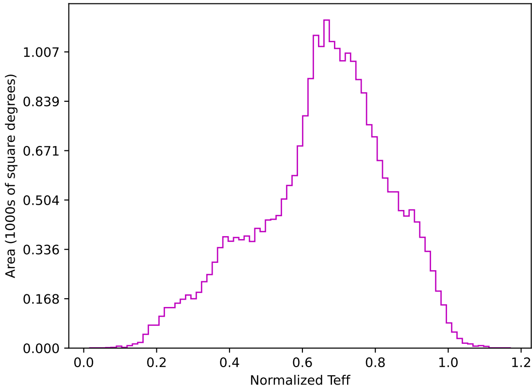
ddf_loaded_fl8_v3.4_10yrs All sky z band: Normalized Teff
