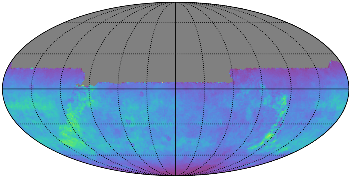
ddf_loaded_fl8_v3.4_10yrs All sky u band: Normalized Teff
