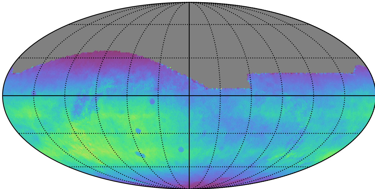
ddf_loaded_fl8_v3.4_10yrs All sky r band: Normalized Teff
