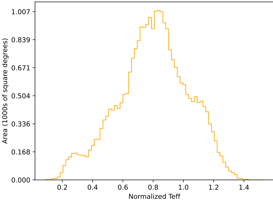
ddf_loaded_fl8_v3.4_10yrs All sky r band: Normalized Teff
