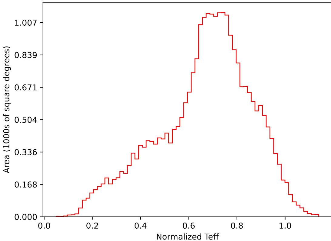
ddf_loaded_fl8_v3.4_10yrs All sky i band: Normalized Teff
