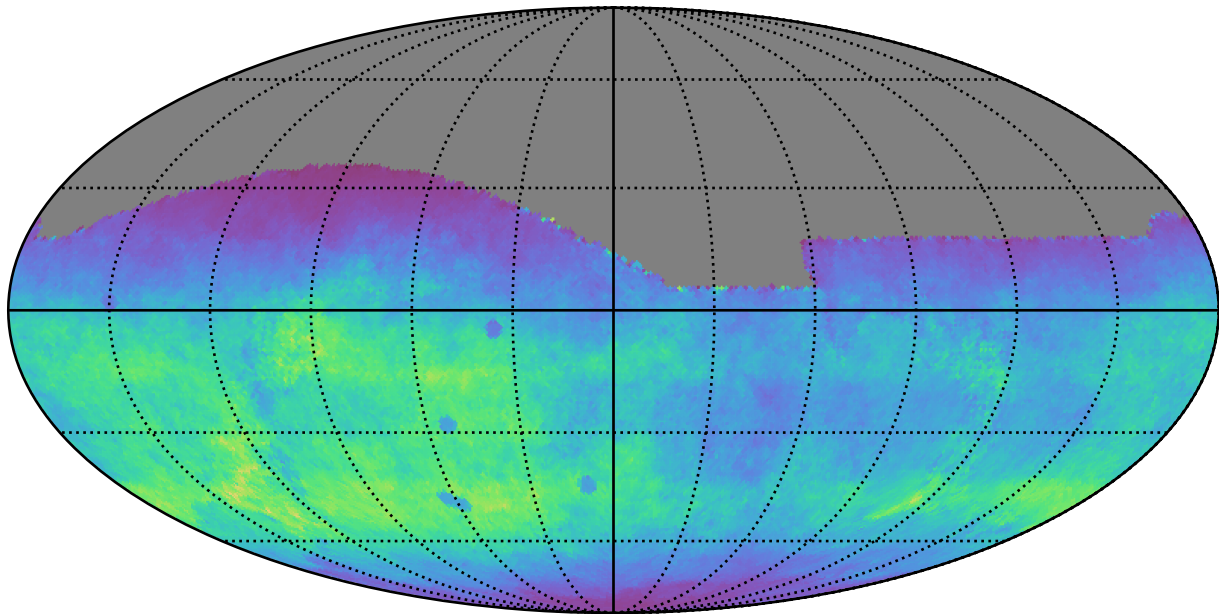
ddf_loaded_fl8_v3.4_10yrs All sky g band: Normalized Teff
