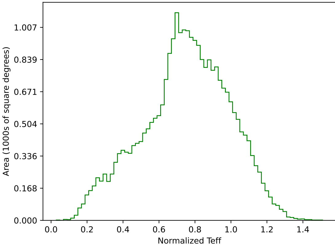
ddf_loaded_fl8_v3.4_10yrs All sky g band: Normalized Teff
