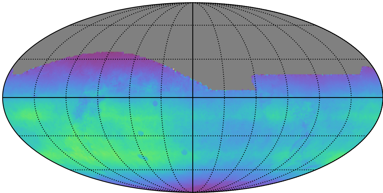
ddf_loaded_fl8_v3.4_10yrs All sky all bands: Normalized Teff
