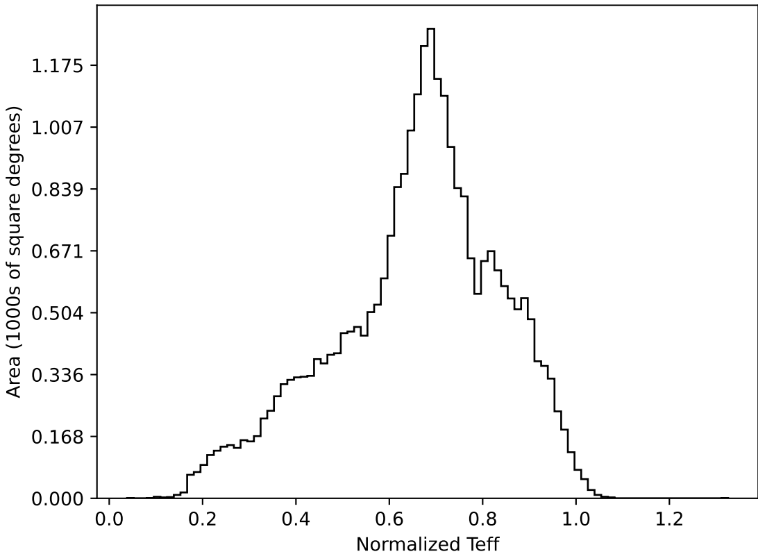
ddf_loaded_fl8_v3.4_10yrs All sky all bands: Normalized Teff
