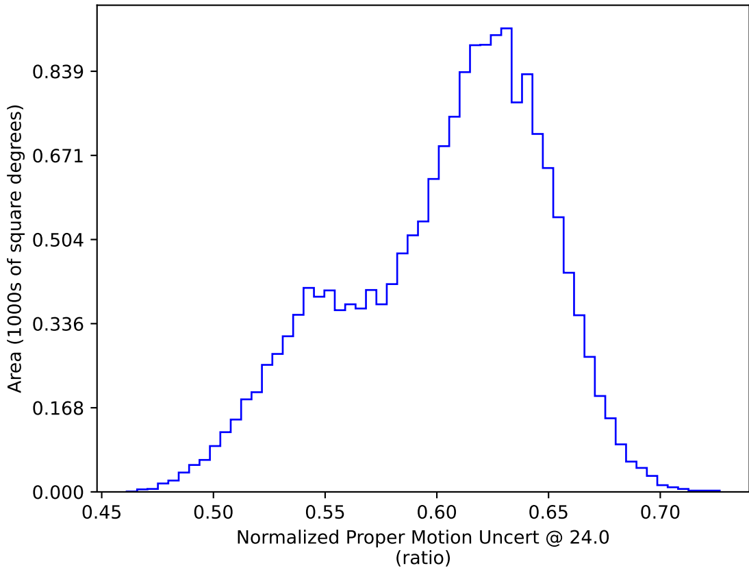
ddf_loaded_fl8_v3.4_10yrs WFD: Normalized Proper Motion Uncert @ 24.0
