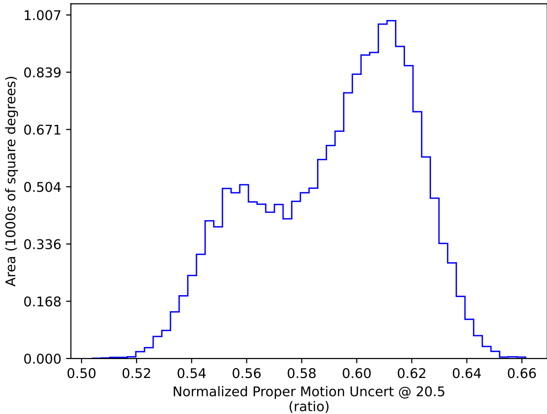
ddf_loaded_fl8_v3.4_10yrs WFD: Normalized Proper Motion Uncert @ 20.5
