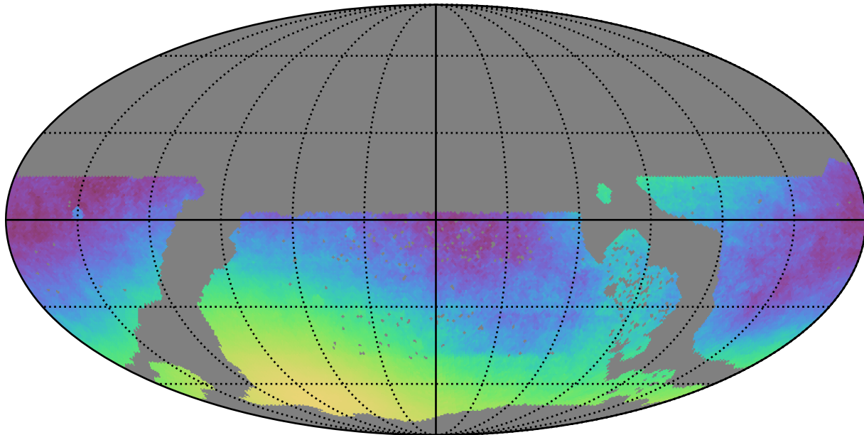
ddf_loaded_fl8_v3.4_10yrs WFD: Normalized Parallax Uncert @ 24.0
