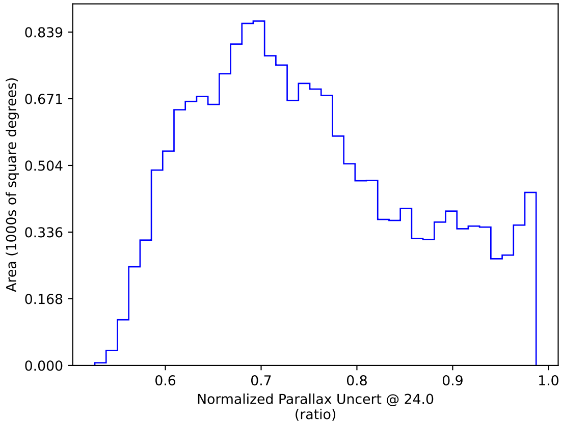
ddf_loaded_fl8_v3.4_10yrs WFD: Normalized Parallax Uncert @ 24.0
