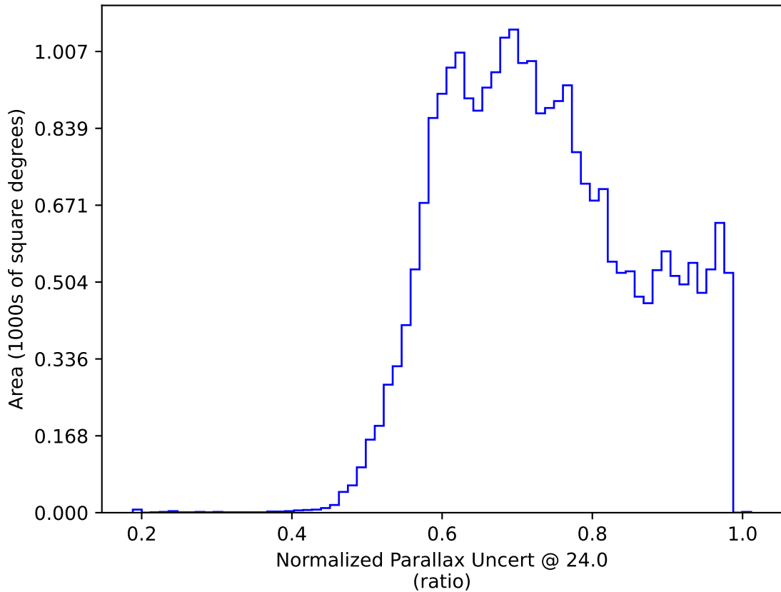
ddf_loaded_fl8_v3.4_10yrs All sky: Normalized Parallax Uncert @ 24.0
