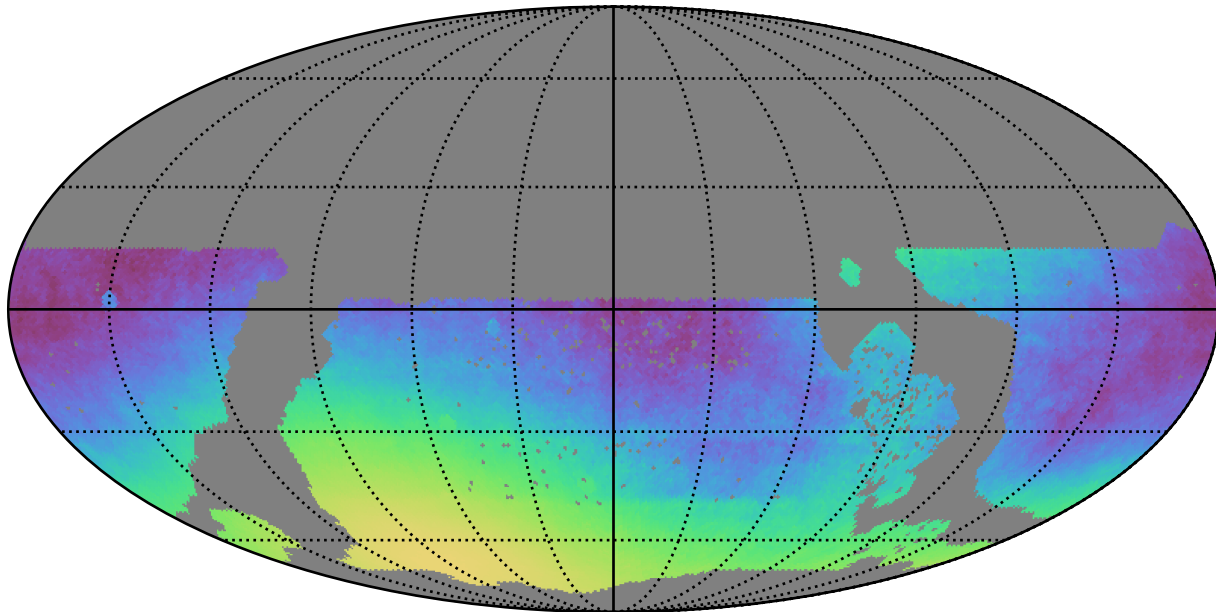
ddf_loaded_fl8_v3.4_10yrs WFD: Normalized Parallax Uncert @ 22.4
