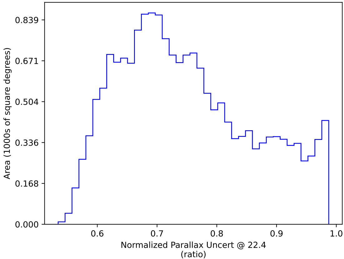
ddf_loaded_fl8_v3.4_10yrs WFD: Normalized Parallax Uncert @ 22.4
