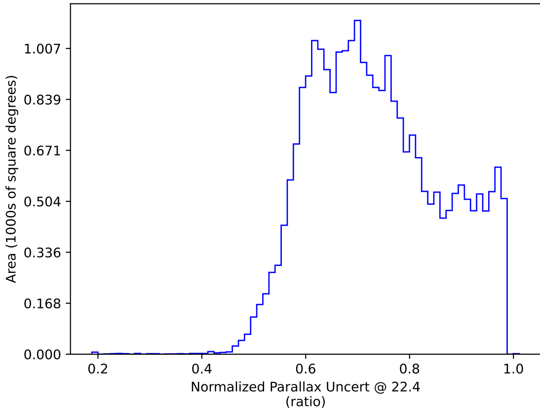
ddf_loaded_fl8_v3.4_10yrs All sky: Normalized Parallax Uncert @ 22.4
