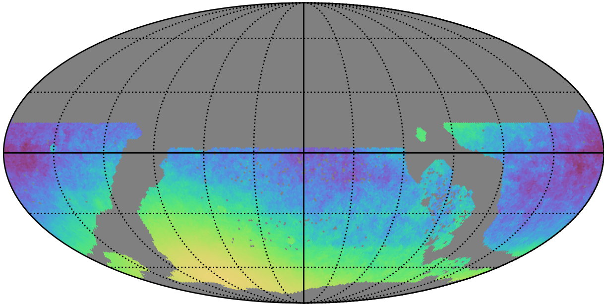
ddf_loaded_fl8_v3.4_10yrs WFD y band only: Normalized Parallax Uncert @ 21.3
