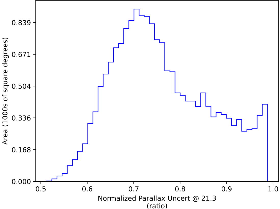
ddf_loaded_fl8_v3.4_10yrs WFD y band only: Normalized Parallax Uncert @ 21.3
