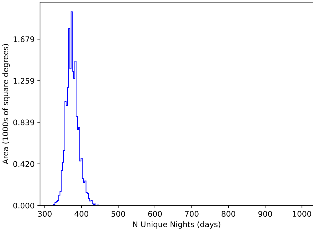
ddf_loaded_fl8_v3.4_10yrs WFD all bands: N Unique Nights
