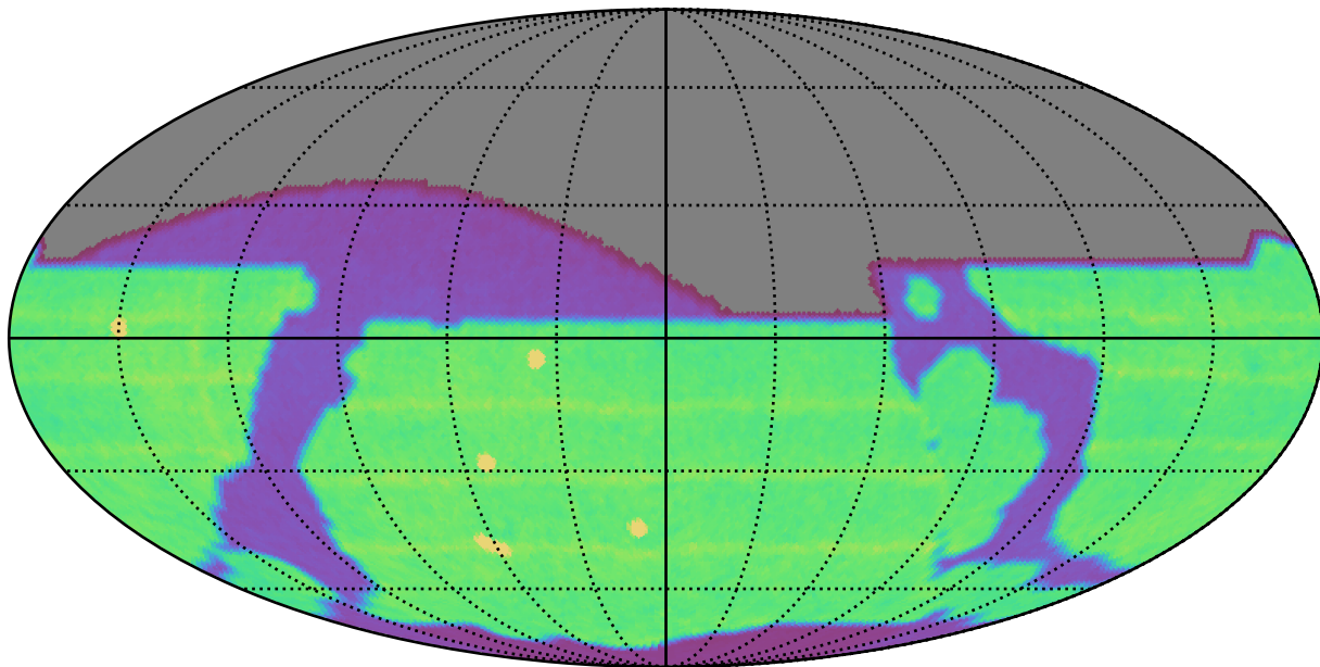
ddf_loaded_fl8_v3.4_10yrs All sky all bands: N Unique Nights
