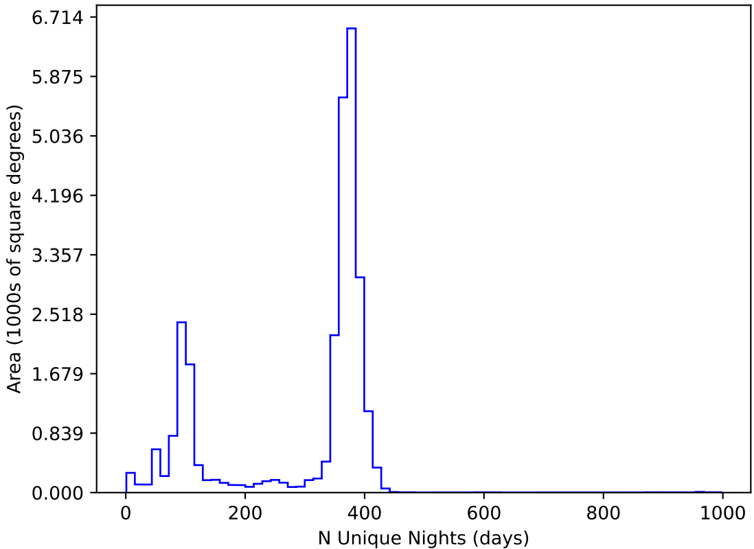
ddf_loaded_fl8_v3.4_10yrs All sky all bands: N Unique Nights
