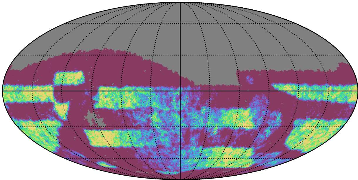
ddf_loaded_fl8_v3.4_10yrs Yr 3-4 z band: NVisits
