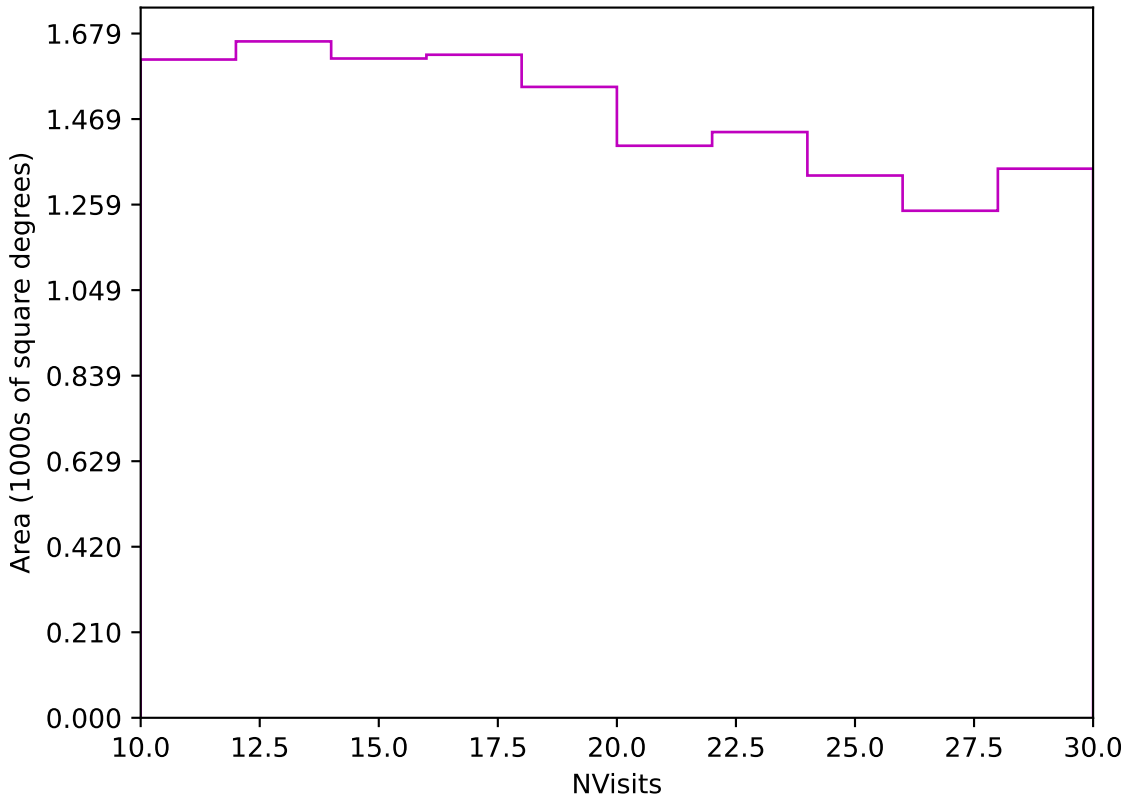
ddf_loaded_fl8_v3.4_10yrs Yr 3-4 z band: NVisits
