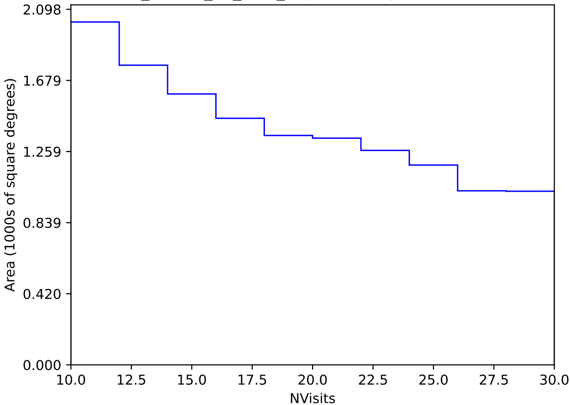
ddf_loaded_fl8_v3.4_10yrs Yr 3-4 y band: NVisits
