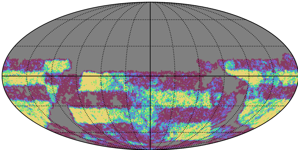
ddf_loaded_fl8_v3.4_10yrs Yr 3-4 u band: NVisits
