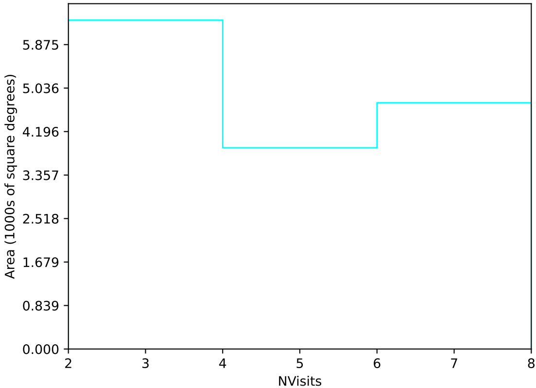
ddf_loaded_fl8_v3.4_10yrs Yr 3-4 u band: NVisits
