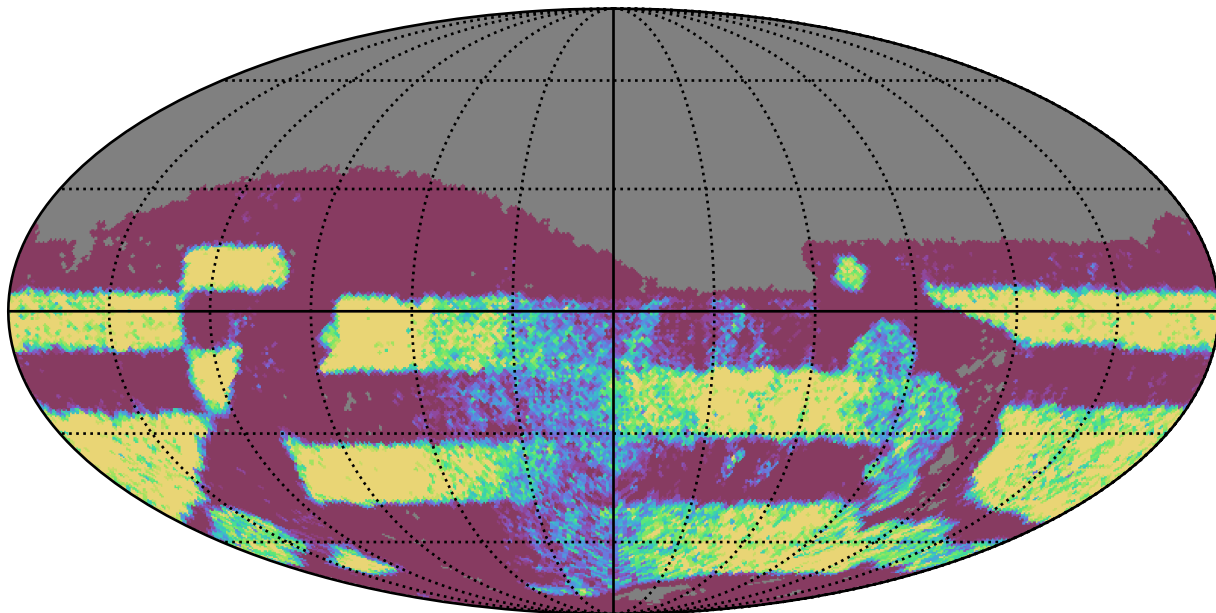
ddf_loaded_fl8_v3.4_10yrs Yr 3-4 r band: NVisits
