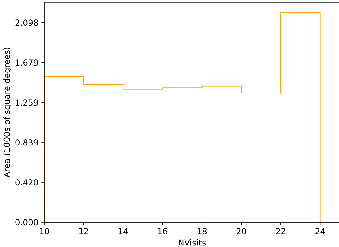
ddf_loaded_fl8_v3.4_10yrs Yr 3-4 r band: NVisits
