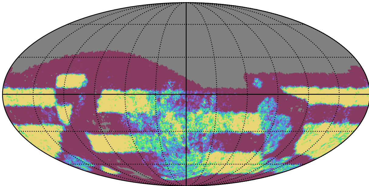
ddf_loaded_fl8_v3.4_10yrs Yr 3-4 i band: NVisits
