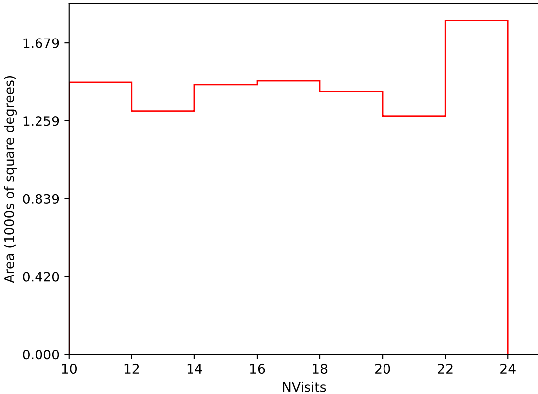
ddf_loaded_fl8_v3.4_10yrs Yr 3-4 i band: NVisits
