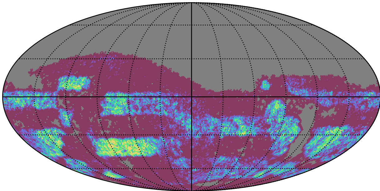
ddf_loaded_fl8_v3.4_10yrs Yr 3-4 g band: NVisits
