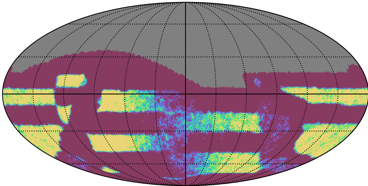
ddf_loaded_fl8_v3.4_10yrs Yr 3-4 all bands: NVisits
