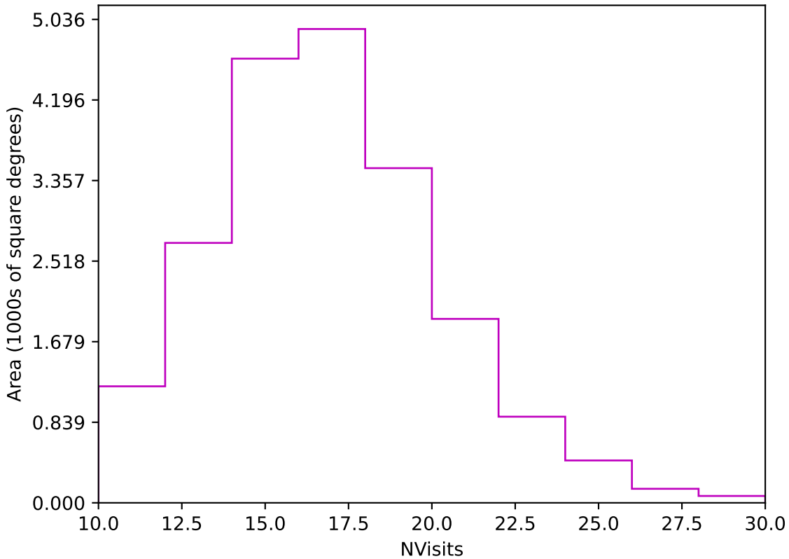
ddf_loaded_fl8_v3.4_10yrs Yr 1 z band: NVisits
