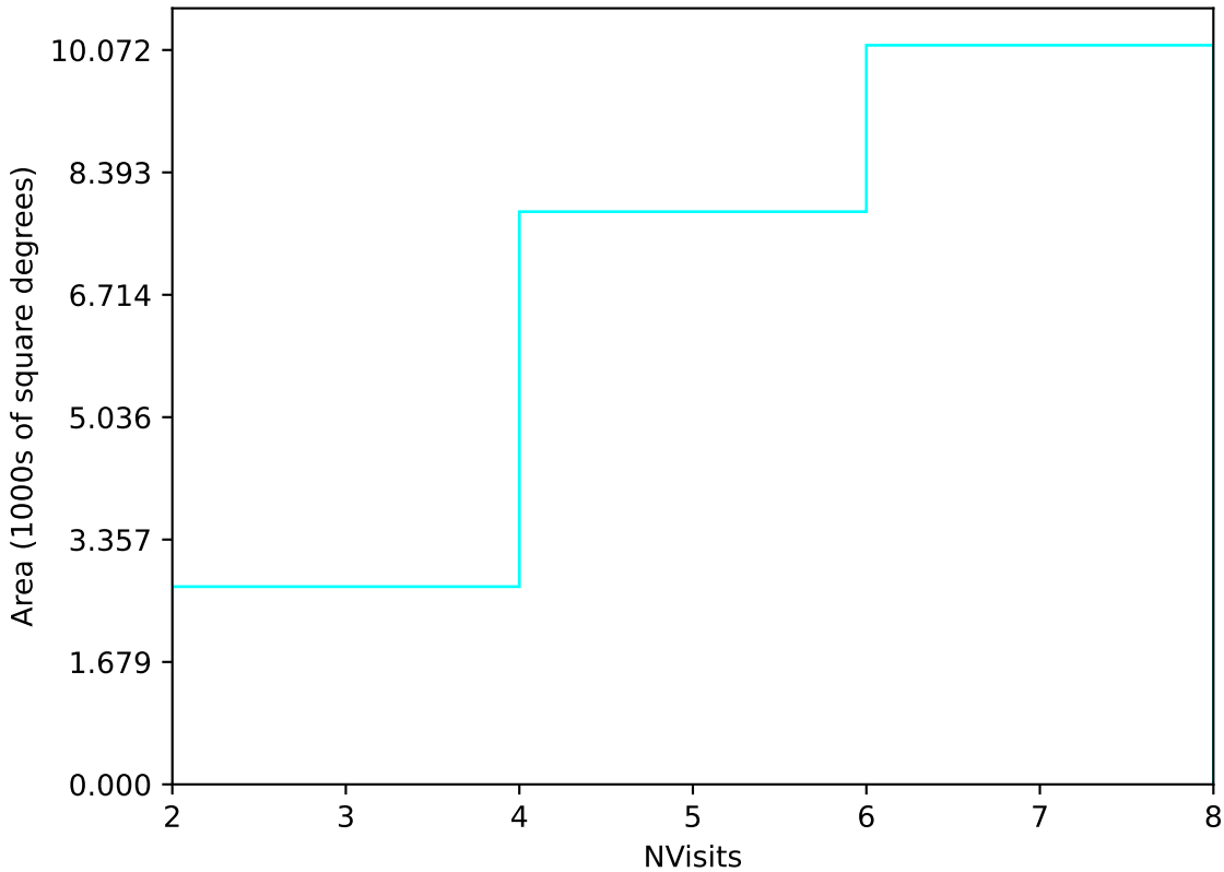
ddf_loaded_fl8_v3.4_10yrs Yr 1 u band: NVisits
