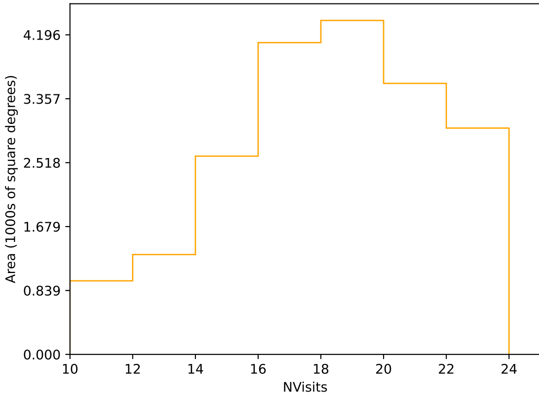
ddf_loaded_fl8_v3.4_10yrs Yr 1 r band: NVisits
