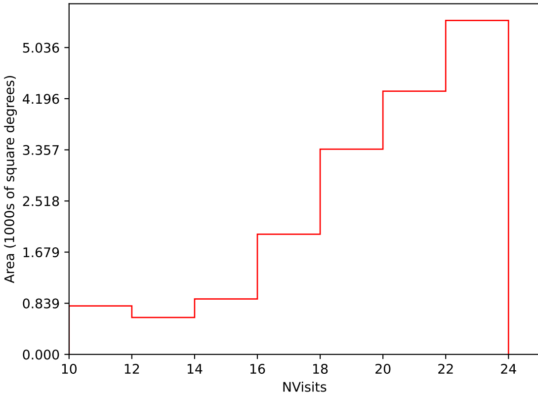
ddf_loaded_fl8_v3.4_10yrs Yr 1 i band: NVisits
