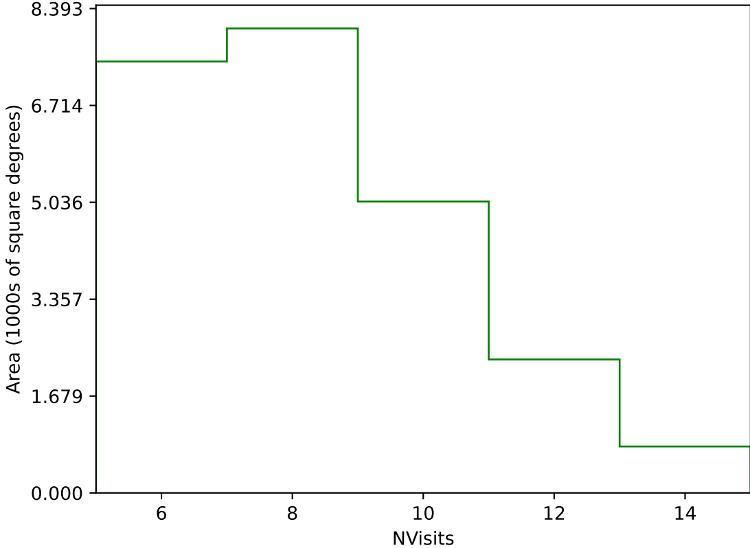
ddf_loaded_fl8_v3.4_10yrs Yr 1 g band: NVisits
