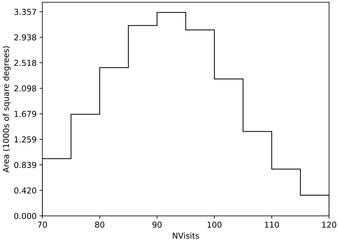
ddf_loaded_fl8_v3.4_10yrs Yr 1 all bands: NVisits
