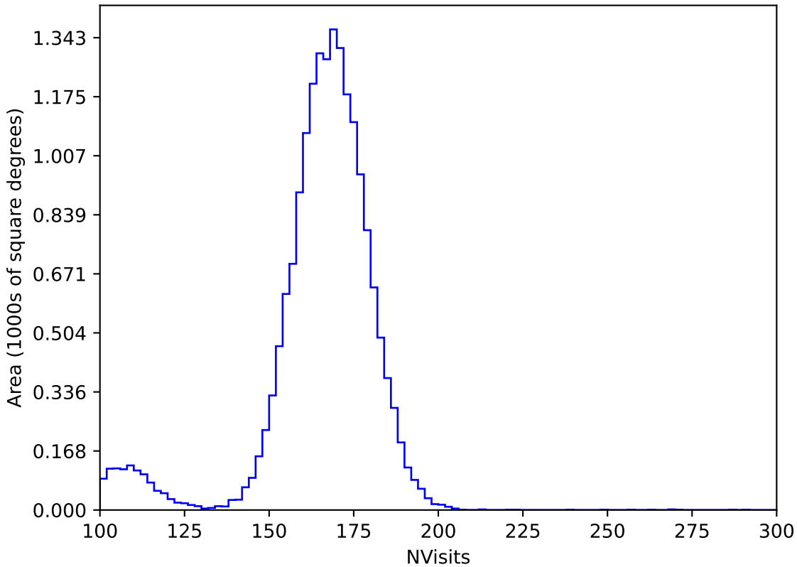
ddf_loaded_fl8_v3.4_10yrs WFD y band: NVisits
