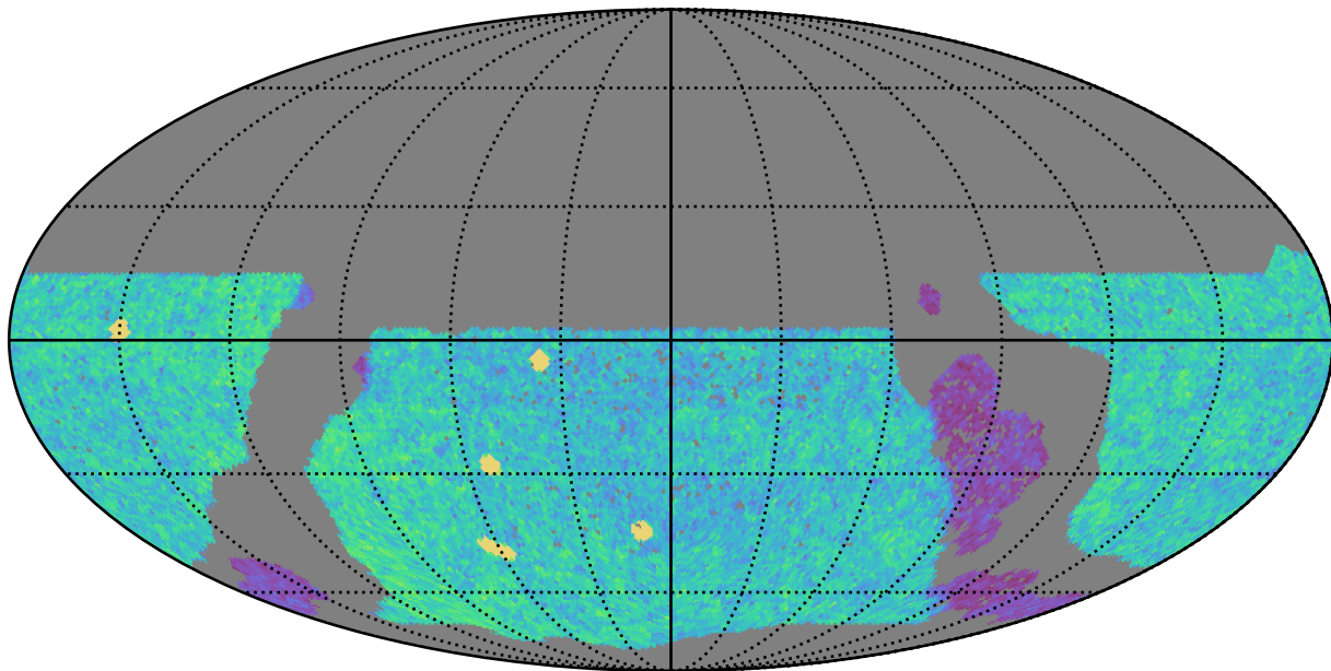
ddf_loaded_fl8_v3.4_10yrs WFD u band: NVisits
