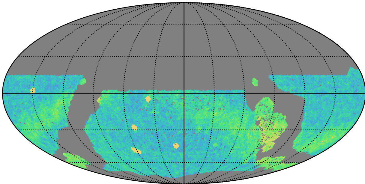
ddf_loaded_fl8_v3.4_10yrs WFD r band: NVisits
