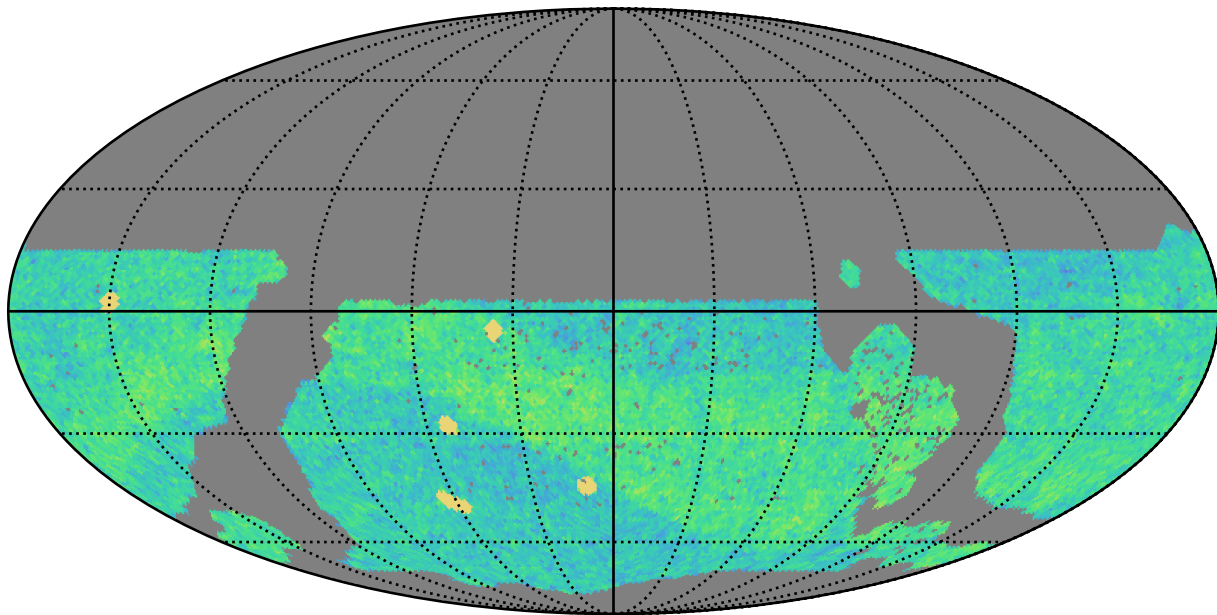
ddf_loaded_fl8_v3.4_10yrs WFD i band: NVisits
