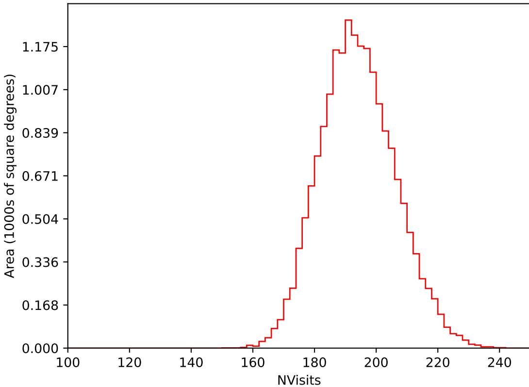
ddf_loaded_fl8_v3.4_10yrs WFD i band: NVisits
