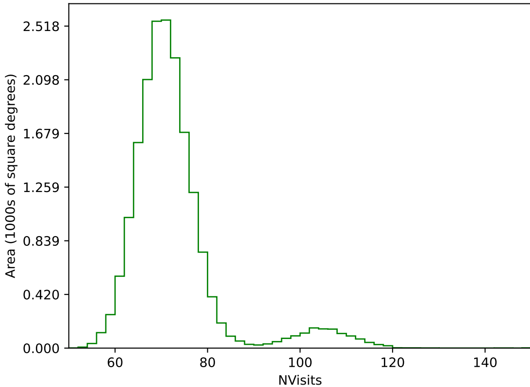
ddf_loaded_fl8_v3.4_10yrs WFD g band: NVisits
