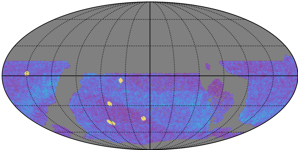
ddf_loaded_fl8_v3.4_10yrs WFD all bands: NVisits
