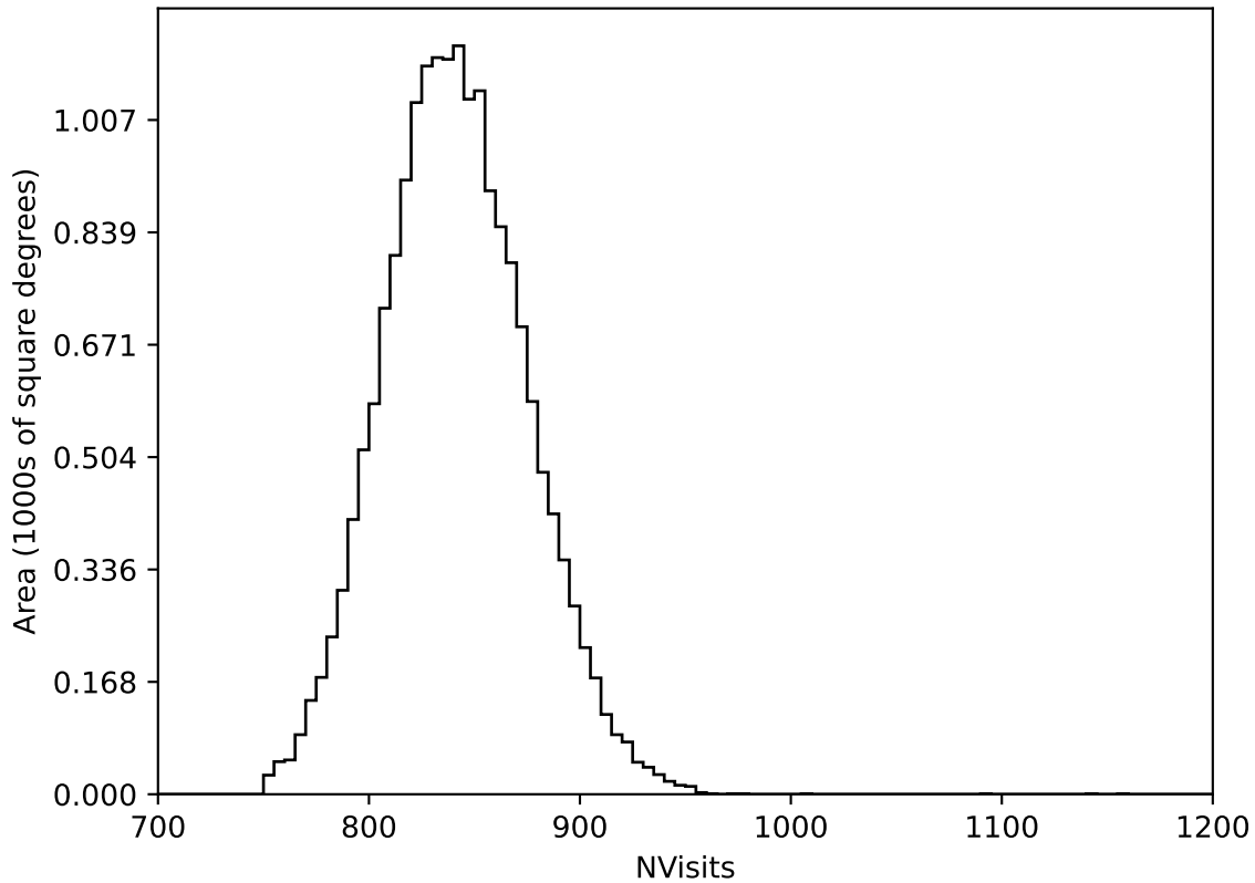
ddf_loaded_fl8_v3.4_10yrs WFD all bands: NVisits
